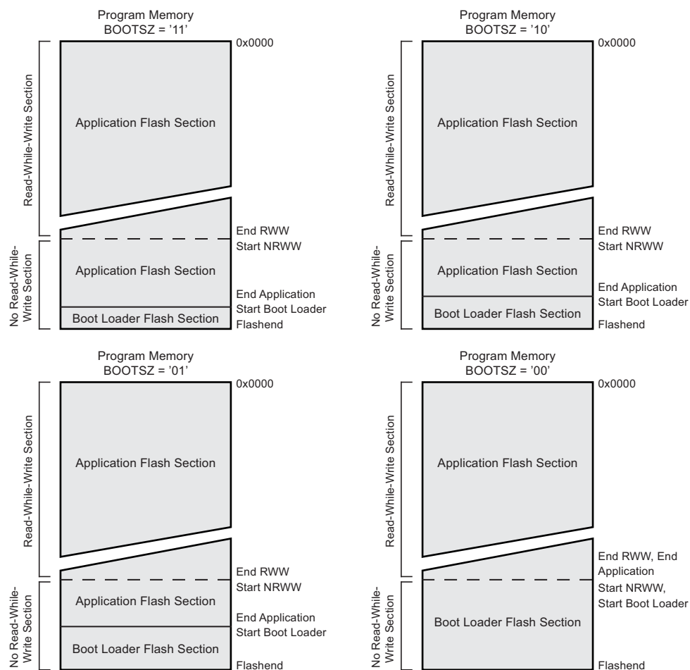
Figure 26-2. Memory Sections
